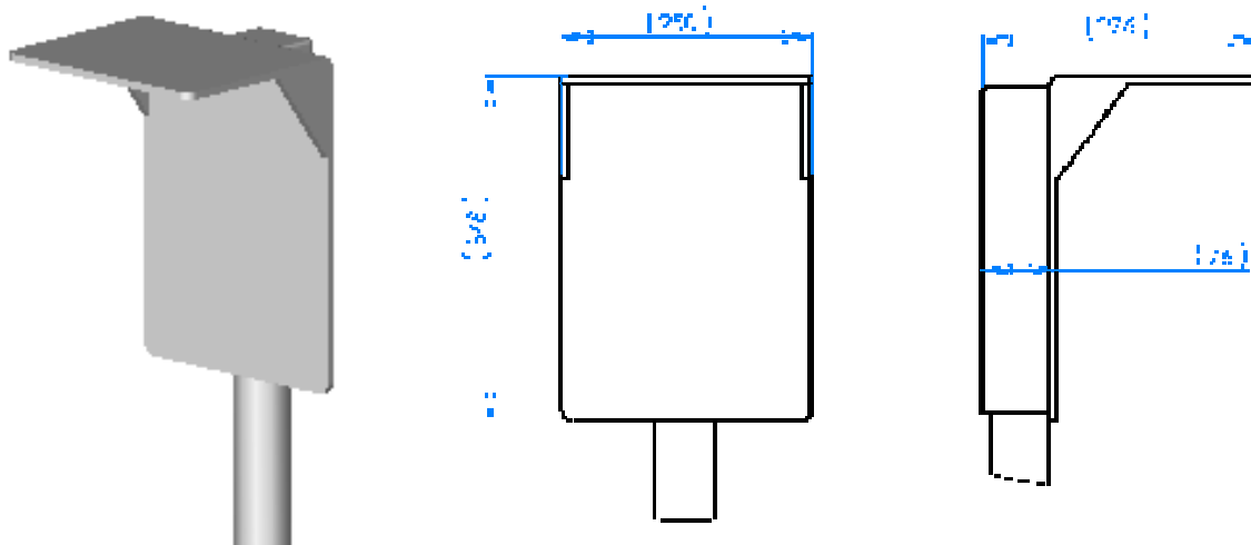
Hood mount for the ACTEON 2053 transmitter ( PON-DPCV-1 for 1 transmitter and PON-PDPCV-2 for 2 transmitters).
